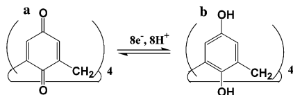
Figure 1. Schematic representation of (a) calix[4]quinone (CQ) and (b) calix[4]hydroquinone (CHQ). CQ can be electrochemically transferred to CHQ by accepting eight electrons and eight protons.
